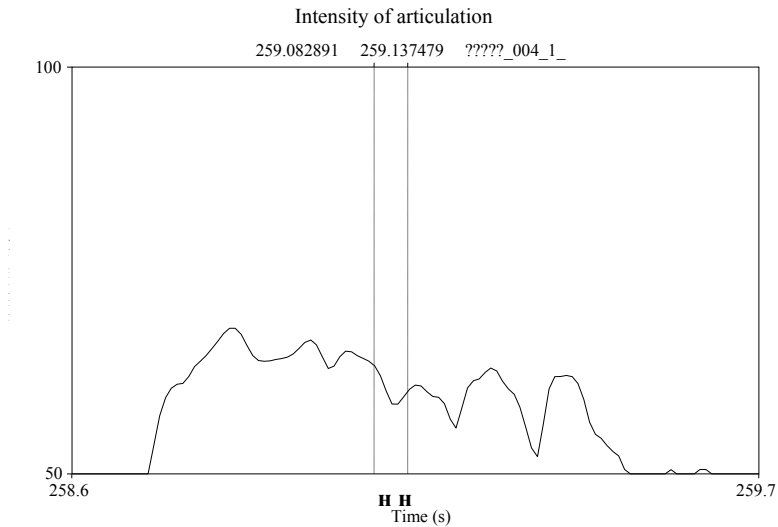
Fig. 5.1. Spectrogram of the word Ukr. ‘romin na seli’
