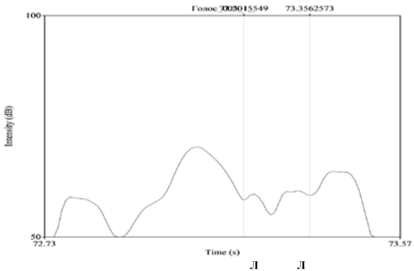
Fig. 5.4. Spectrogram of the word Ukr. 'цвiдцю'
