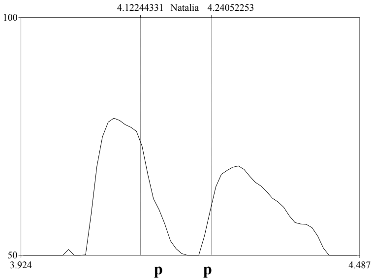
Fig. 6.3. Spectrogram of the word Germ. 'Suppe'
