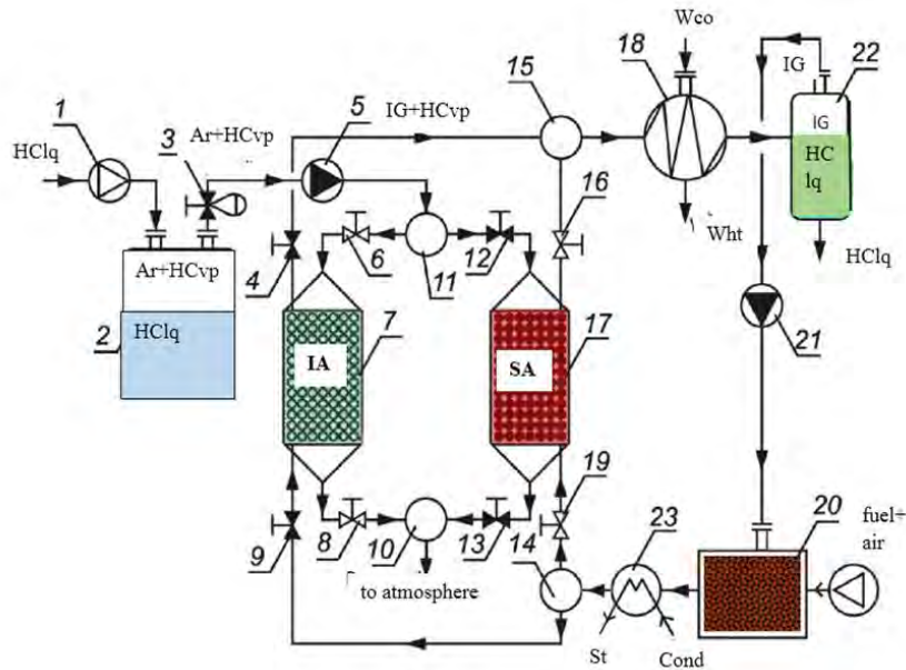
Figure 7. Schematic diagram of vapor recovery hydrocarbons.
