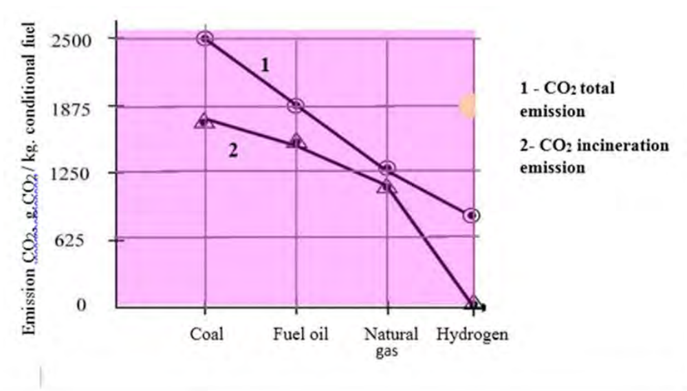
Figure 5. Emissions of carbon dioxide depending on the type of fuel burned
