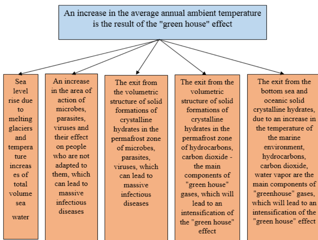
Figure 3. The impact of an increase in the average annual temperature of the environment on the negative impact on ecosystems, biota, biomes, biosphere, humans
