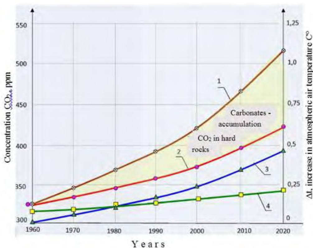
Figure 2 – Change in the concentration of carbon dioxide and the average annual increase in atmospheric air temperature depending on time (years).
