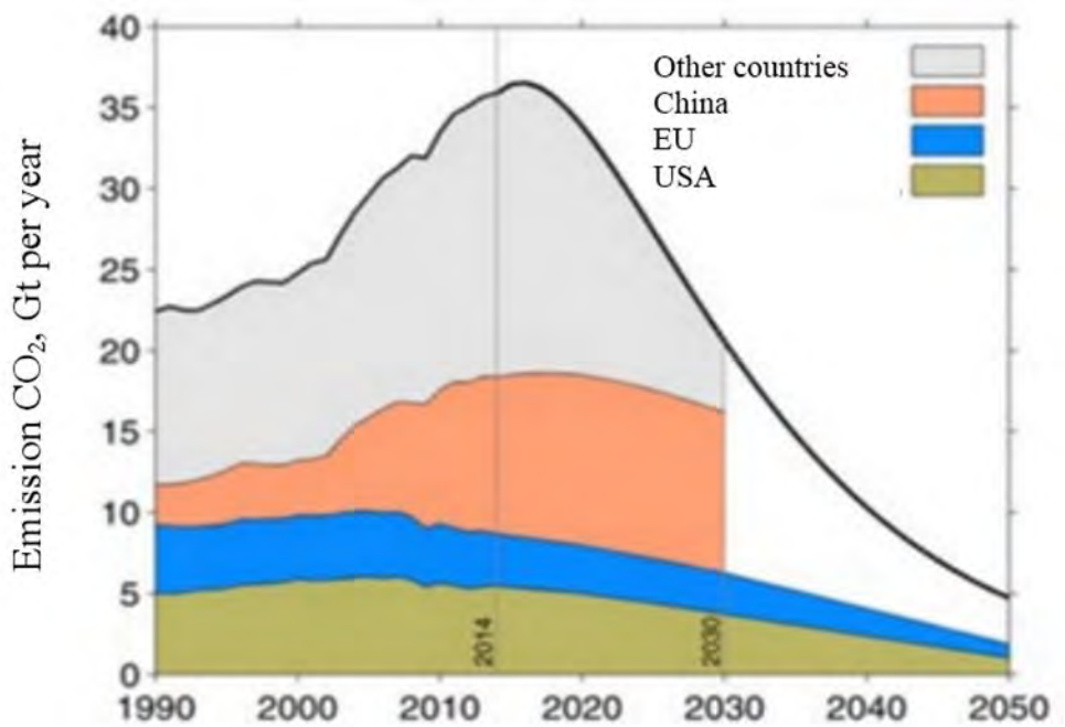
Figure 6. Dependence of the emission of carbon dioxide into the air basin depending on the time 24
