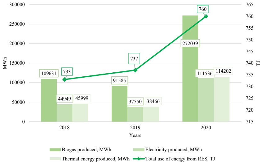
Figure 18. Production indicators of the MHP biogas complex in 2018-2020
